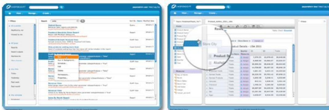
Σχήμα 2-2: Jasper Reporting
