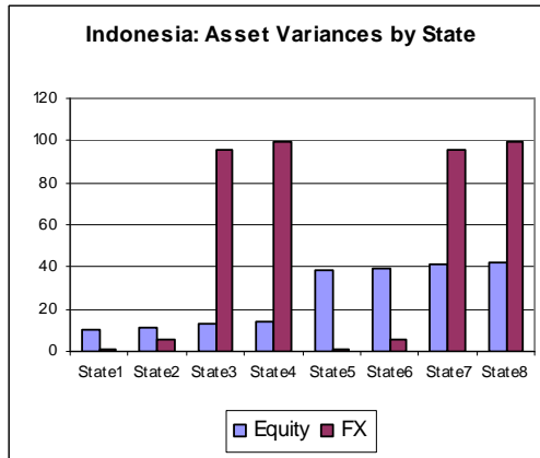
Figure 7. Conditional Variances by state
