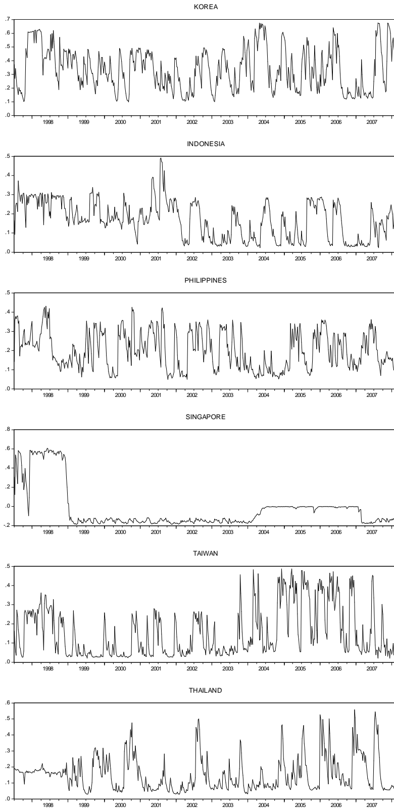
Figure 6. Contribution of pure contagion to conditional correlations
