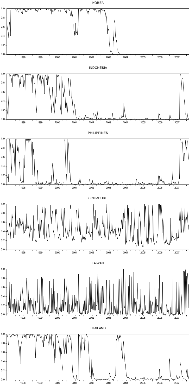
Figure 2. Filter Probabilities of high volatility common shocks
