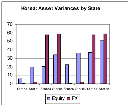
Figure 7. Conditional Variances by state
